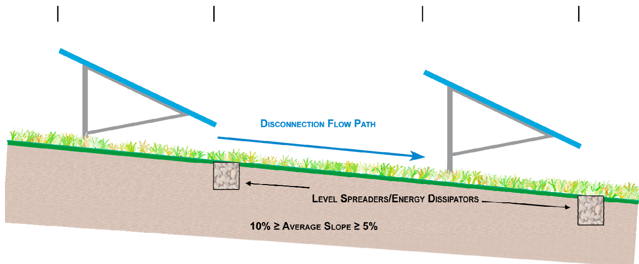
Figure 2. Typical Installation – Slope \geq 5\% but \leq 10\%
